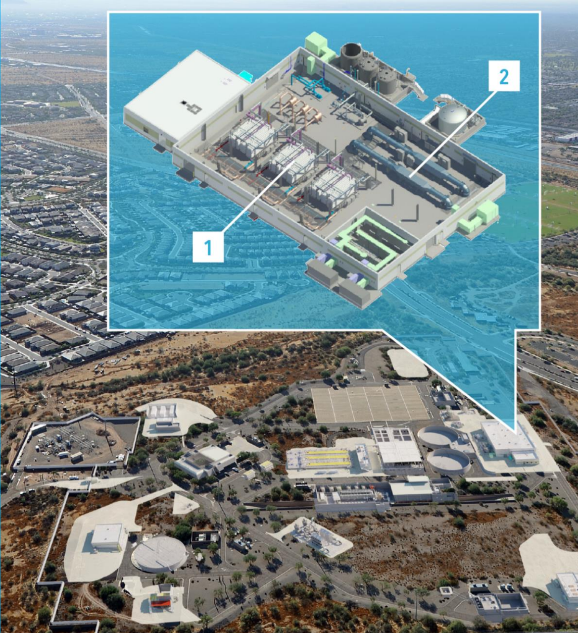
(1) Reverse Osmosis and (2) UV Advanced Oxidation technologies.
